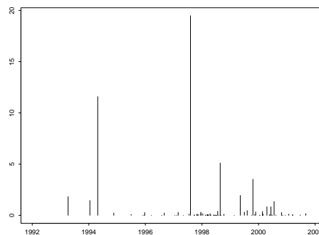
Figure 2: Operational risk losses, Type 2, n = 80 .
